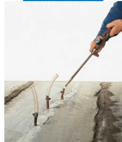
Restoring horizontal structure by injection with Epojet
