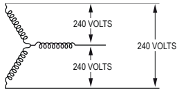
THREE-PHASE, THREE-WIRE (WYE) A
